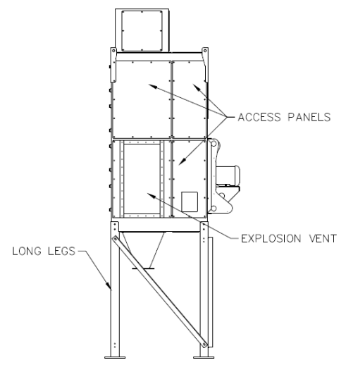
FRP8 EQUIPPED WITH LONG LEGS/HOPPER—INLET PLENUM - EXPLOSION VENT
