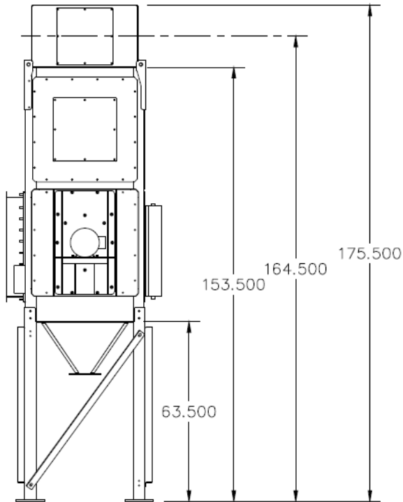
FRP8 EQUIPPED WITH LONG LEGS/HOPPER—INLET PLENUM - EXPLOSION VENT
