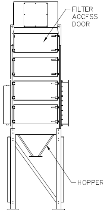
FRP8 EQUIPPED WITH LONG LEGS/HOPPER—INLET PLENUM - EXPLOSION VENT
